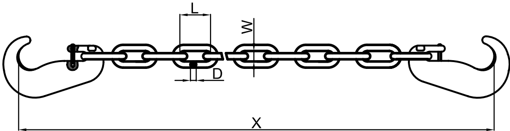
Lashing chain with C HOOK / EL FOOT C-1B
