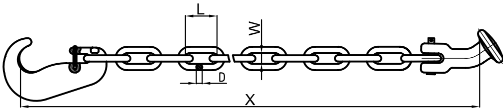
Lashing chain with C HOOK / EL FOOT C-1B
