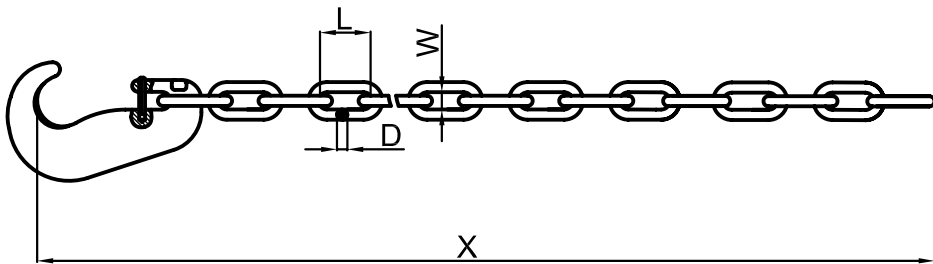
Lashing chain with single C HOOK / C-1C
